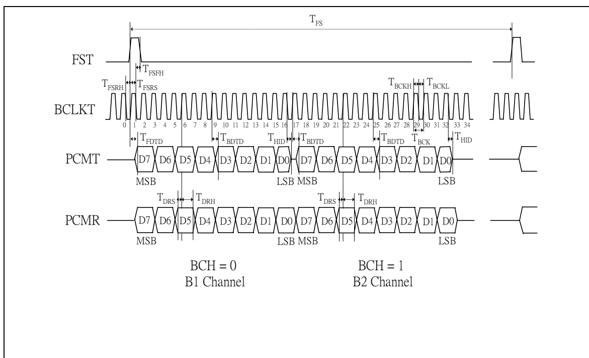
Figure 8.4 GCI PCM Timing
